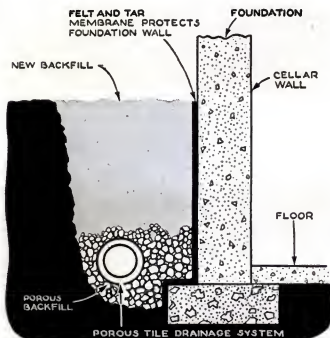
Only sure cure for bad leakage is to encase basement in a "membrane" of felt and tar.
